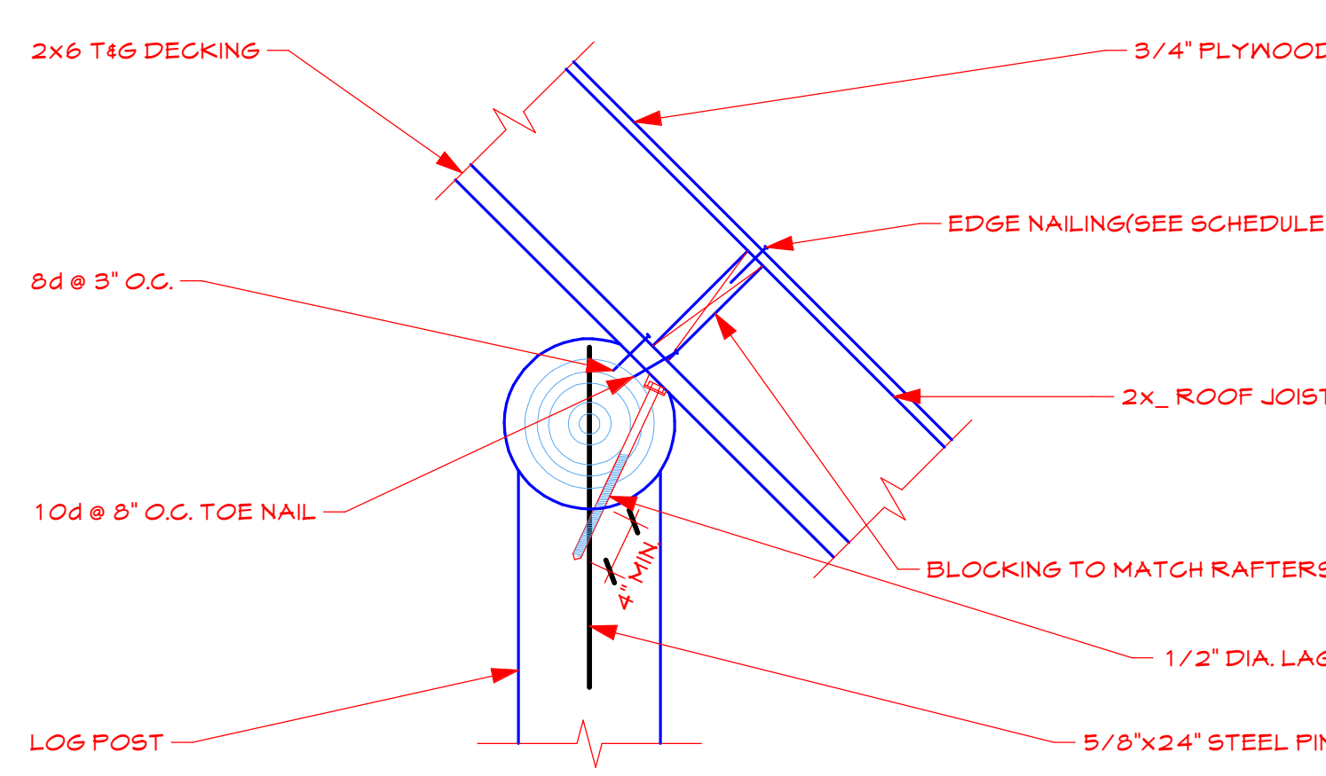
D28 ROOF TO PURLIN CONNECTION SCALE: 1" = 1'-0"
