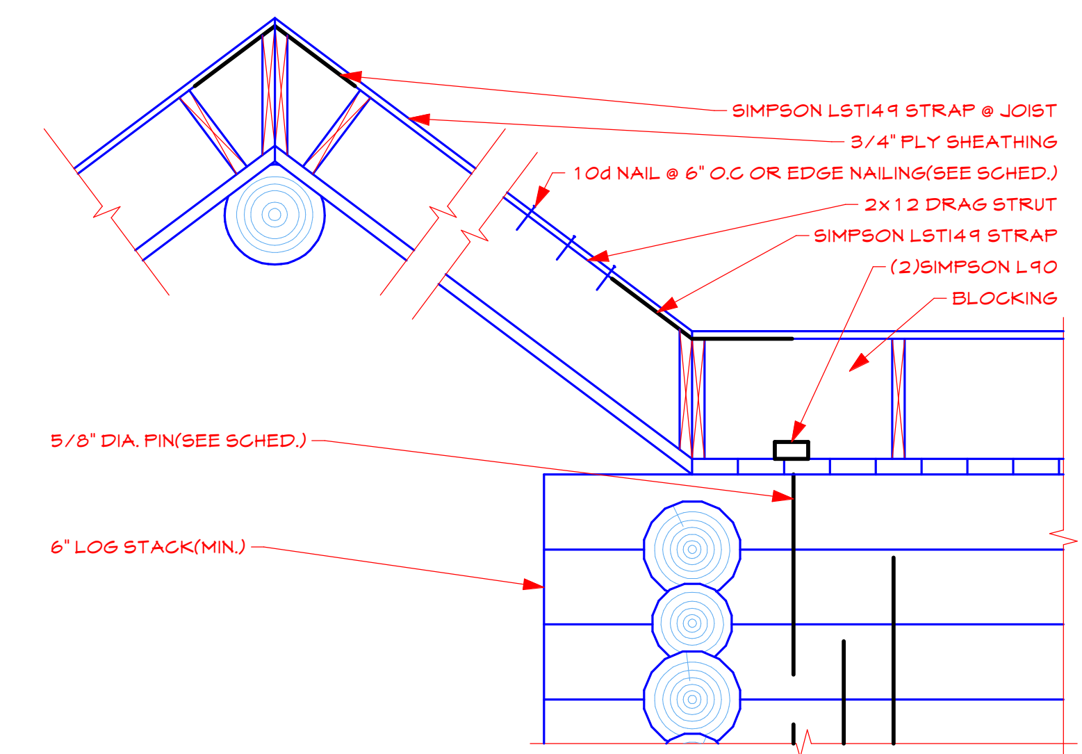
D31 ROOF TO WALL CONNECTION SCALE: 3/4" = 1'-0"
