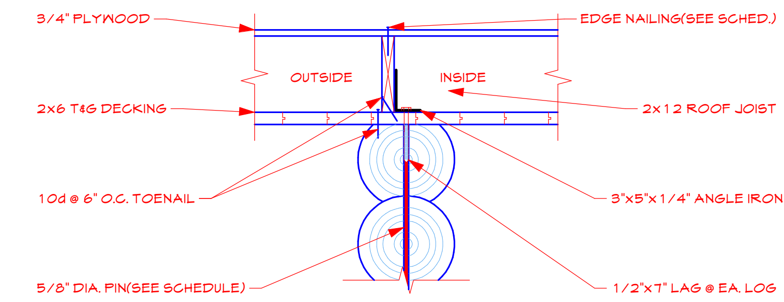
D30 ROOF TO GABLE CONNECTION SCALE: 1" = 1'-0"
