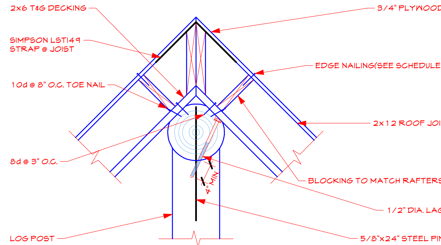
D27 ROOF TO RIDGE CONNECTION SCALE: 1" = 1'-0"
