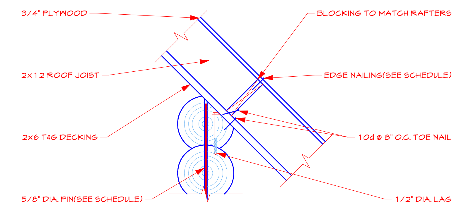
D29 ROOF TO PLATE CONNECTION SCALE: 1" = 1'-0"
